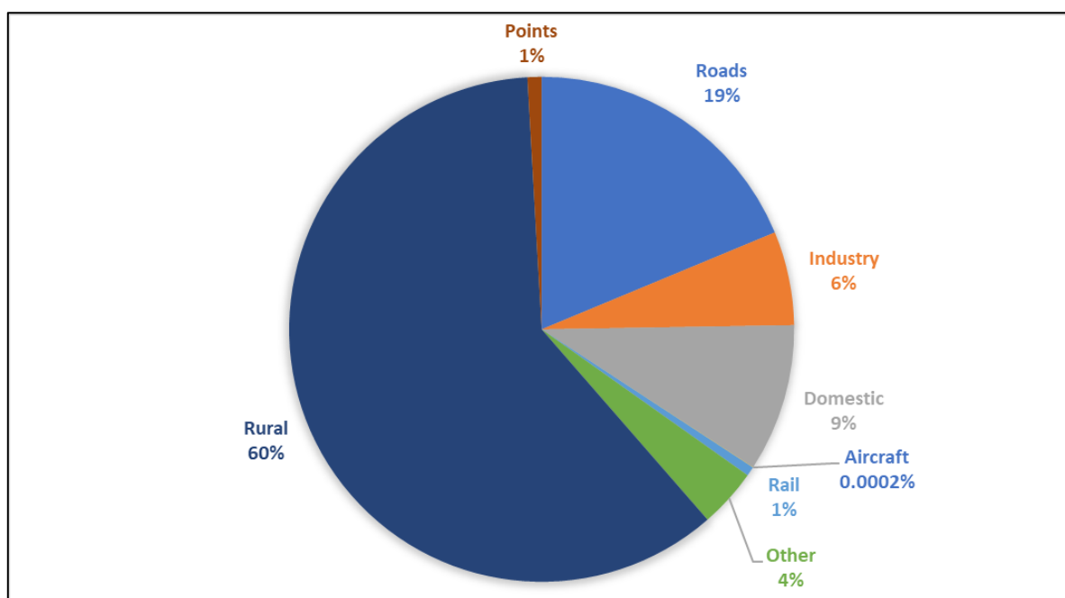
Figure 3-7: Average source apportionment for NO x concentrations in Chipping Norton AQMA based on Defra background maps
